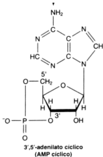
(b) Hydrolysis of ATP
