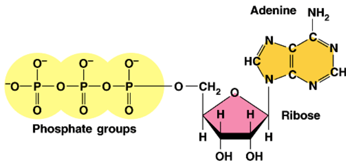
(a) Structure of adenosine triphosphate
