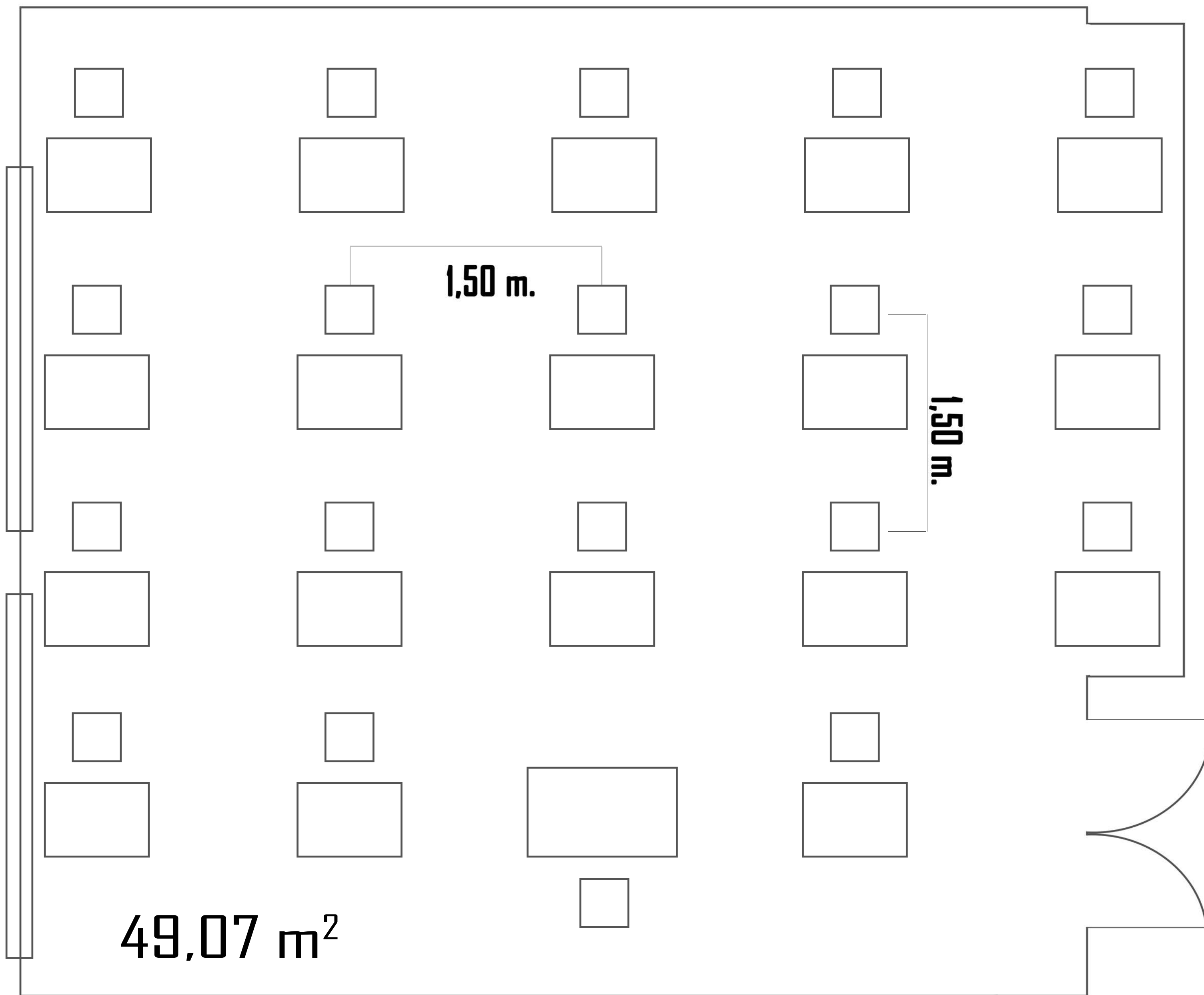
Plano aula IES As Bizocas
