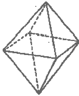
Octaedro
