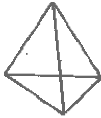
Tetraedro
