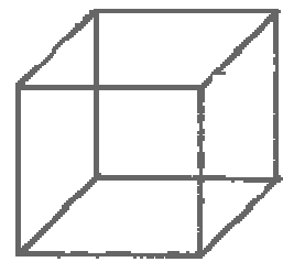
Hexaedro
